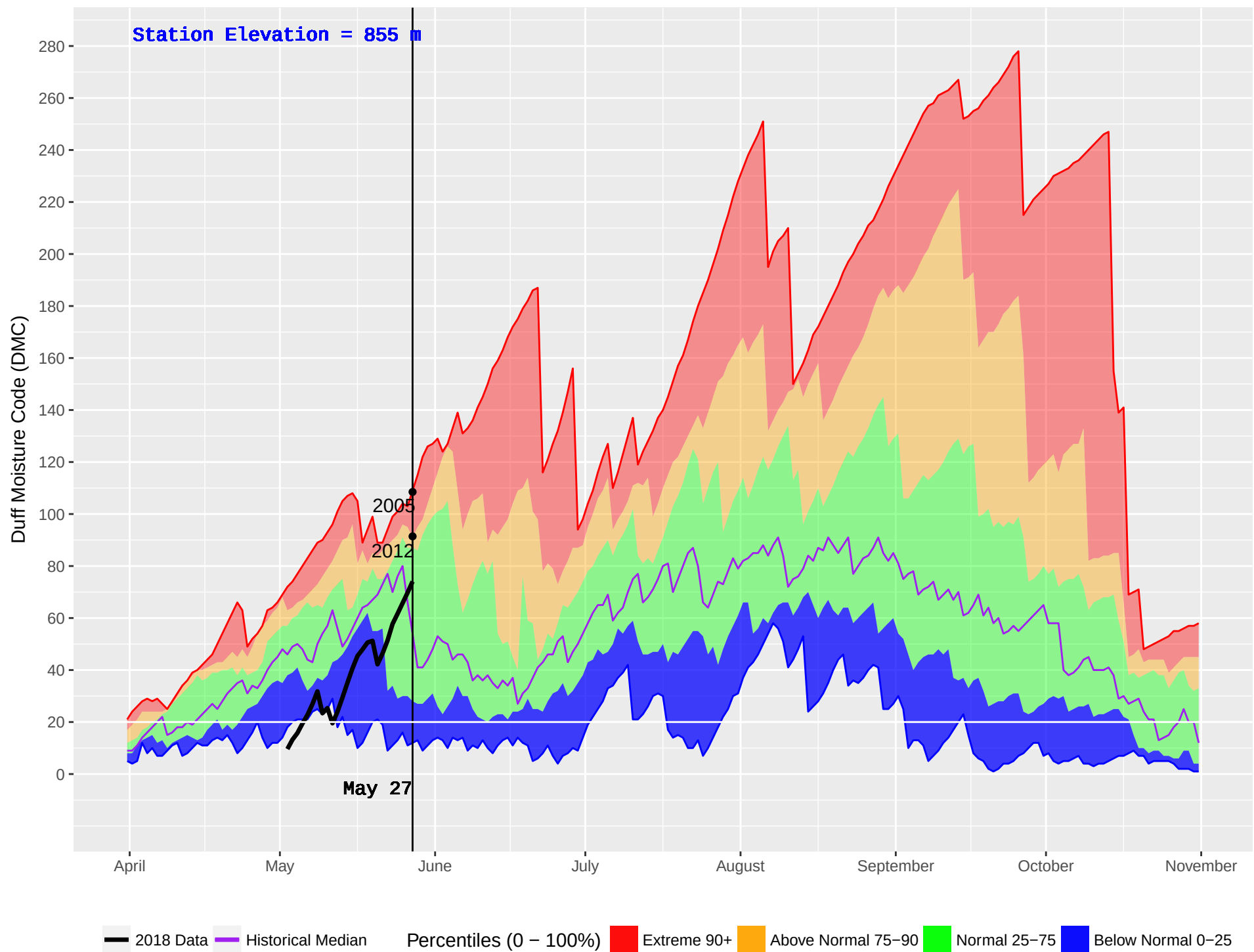
AUGUST LAKE (836) : Historical (2003–2016) and Current (2018) Noon Duff Moisture Code (DMC)
