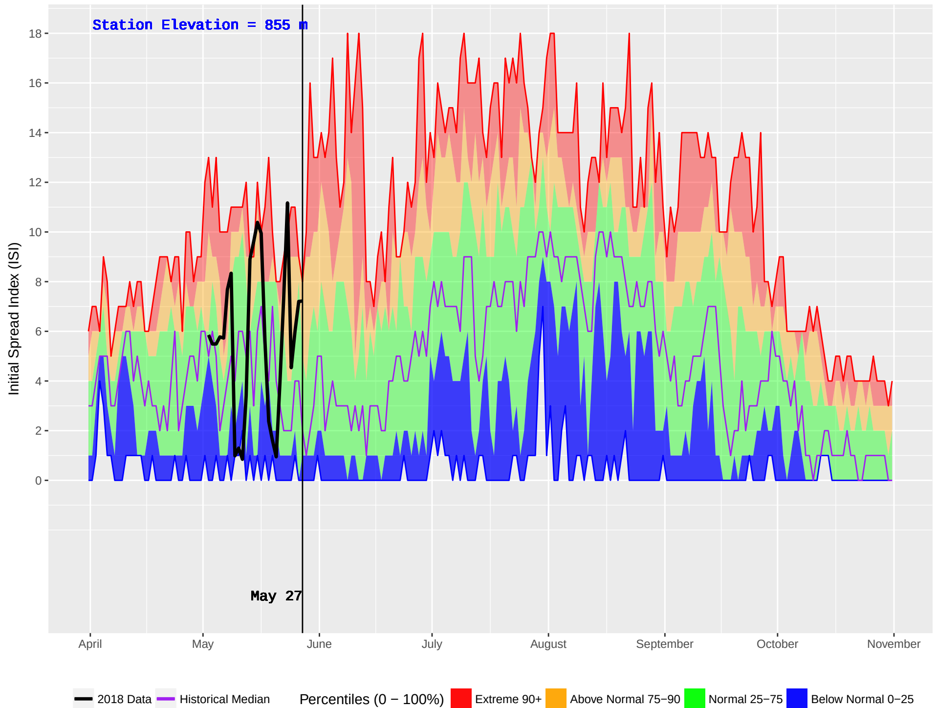
AUGUST LAKE (836) : Historical (2003–2016) and Current (2018) Noon Initial Spread Index (ISI)
