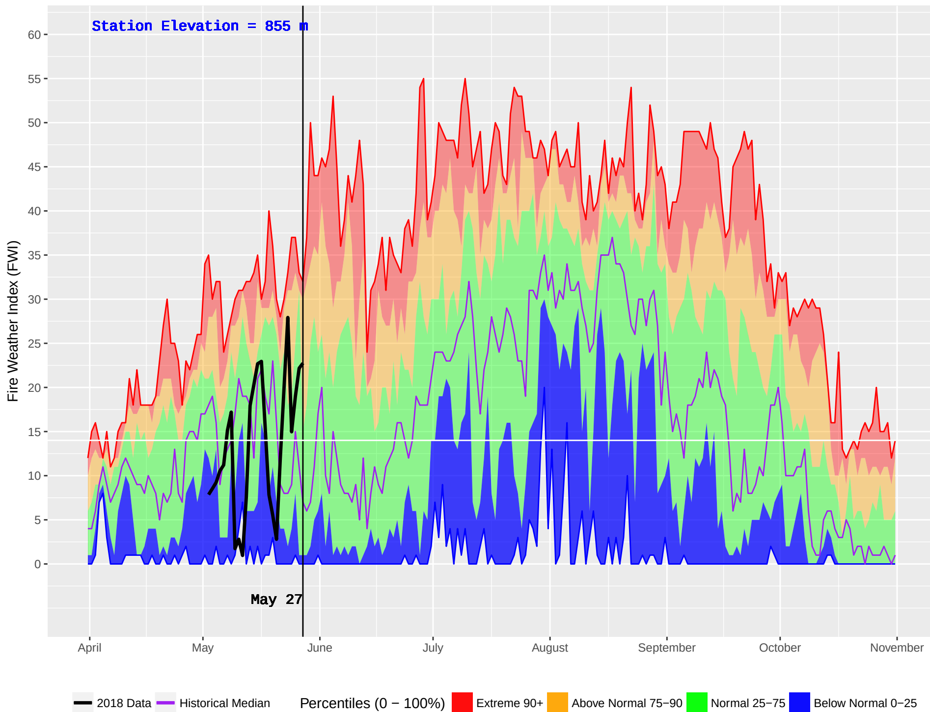
AUGUST LAKE (836) : Historical (2003–2016) and Current (2018) Noon Fire Weather Index (FWI)
